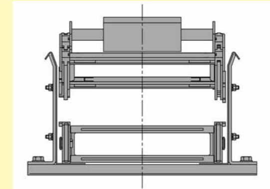
Install the mobile point of the cable chain aligning it exactly to the longitudinal travel distance in such a way so that during its movement it does not touch the internal part of the guide channel (Fig. A).
