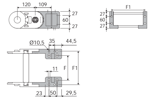
Fig. A The chain can be fixed frontally, inner or outer radius. (Fig A)
