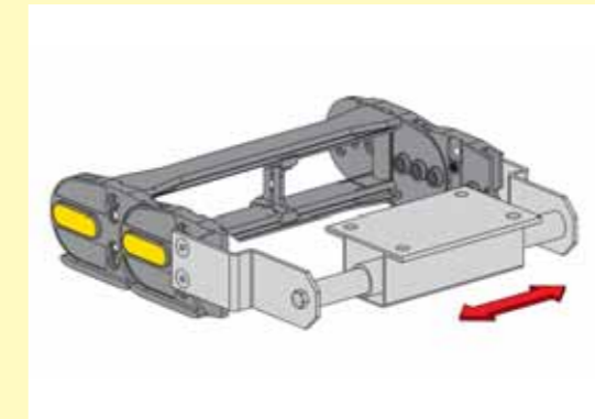
To facilitate this operation Brevetti Stendalto has developed and created a special movable end bracket which guarantees a perfect alignment between the chain and the towing arm (Fig. B).
